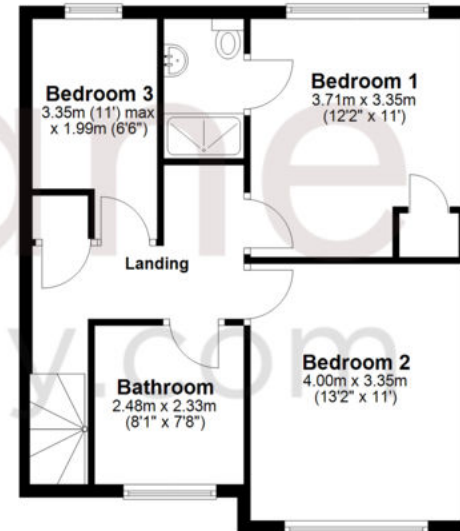
First Floor Approx. 50.7 sq. metres (545.5 sq. feet)
